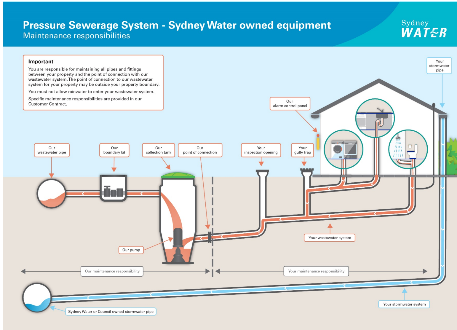
Figure 5: Typical pressure sewerage equipment maintenance responsibilities – Sydney Water owned equipment
