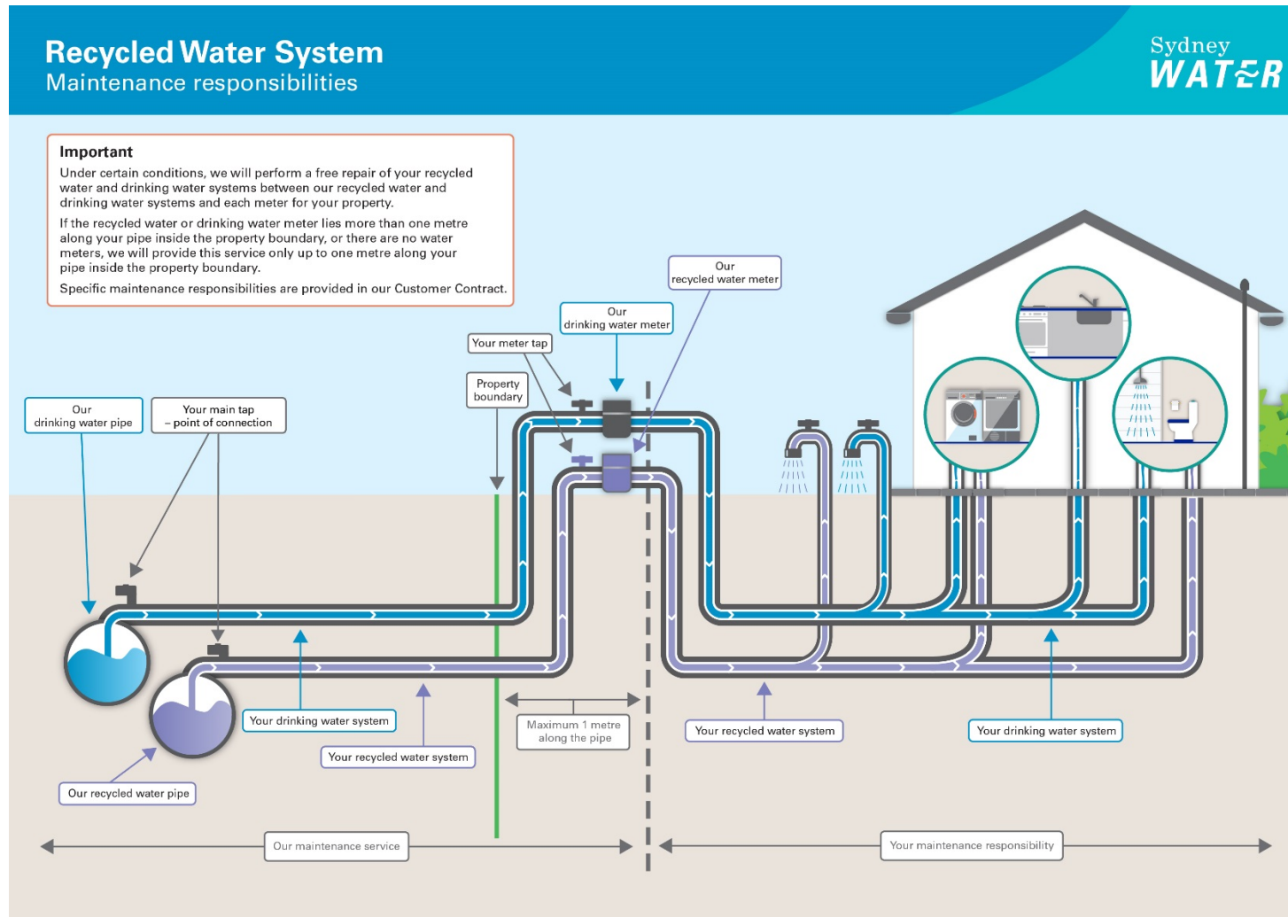
Figure 2: Typical recycled water system maintenance responsibilities
