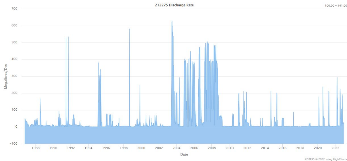
Figure 5-2: Graph of median stream flow at 212275 Wingecarribee River at Sheepwash Bridge
