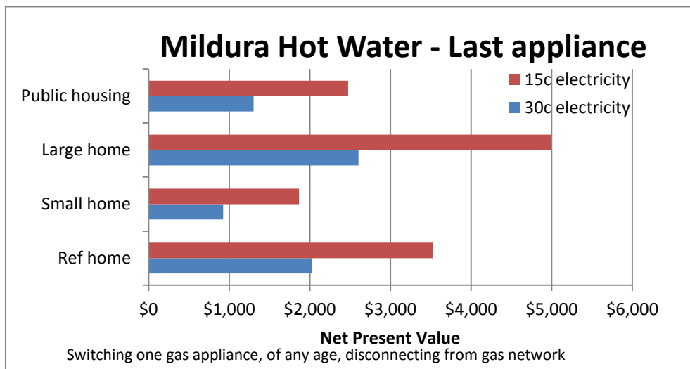
Figure 3-6: Sensitivity to availability of Off-Peak, Mildura, Hot Water, Last Appliance
