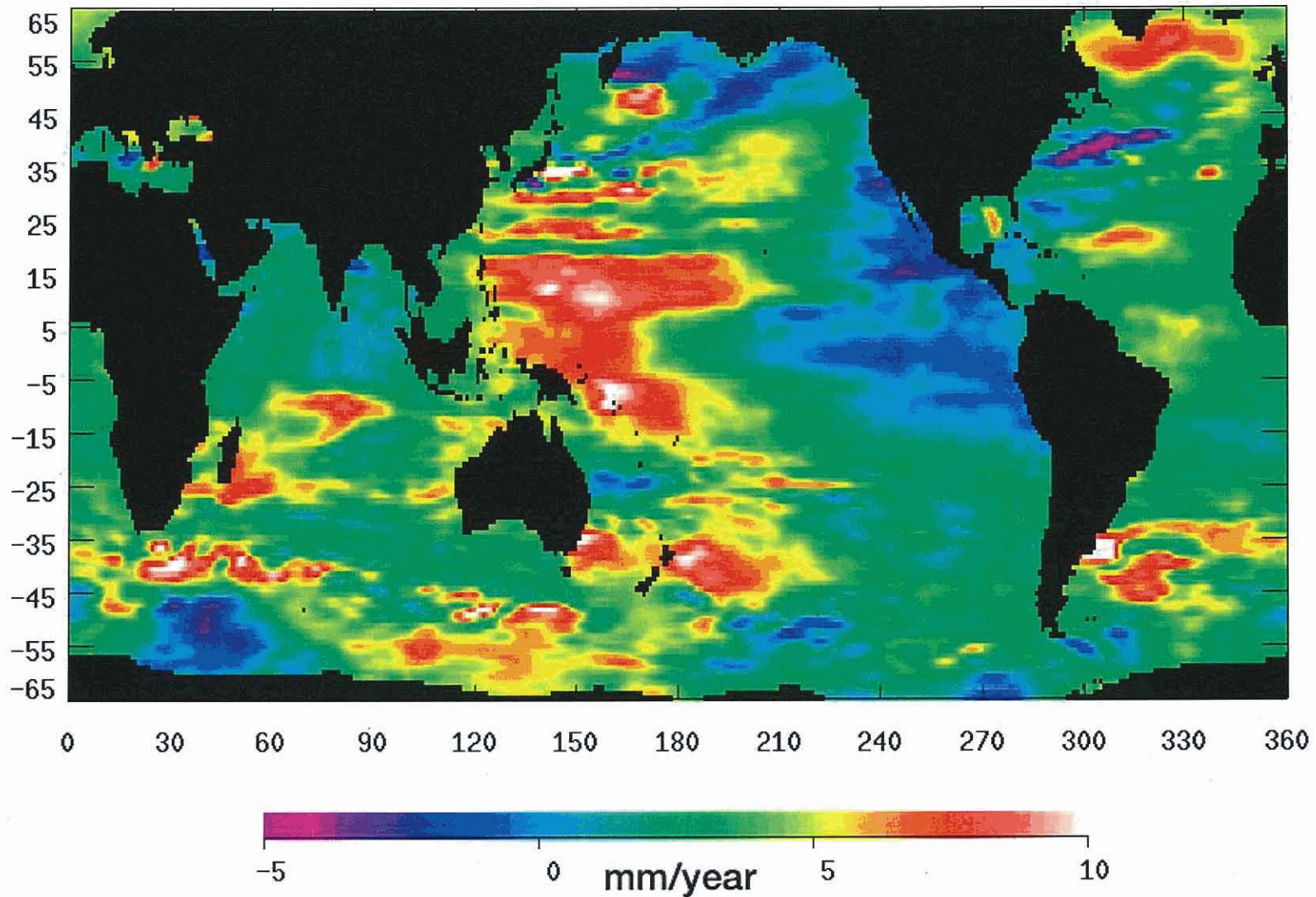
Figure 3 – Regional variations in recorded sea level rise (source: NASA)
