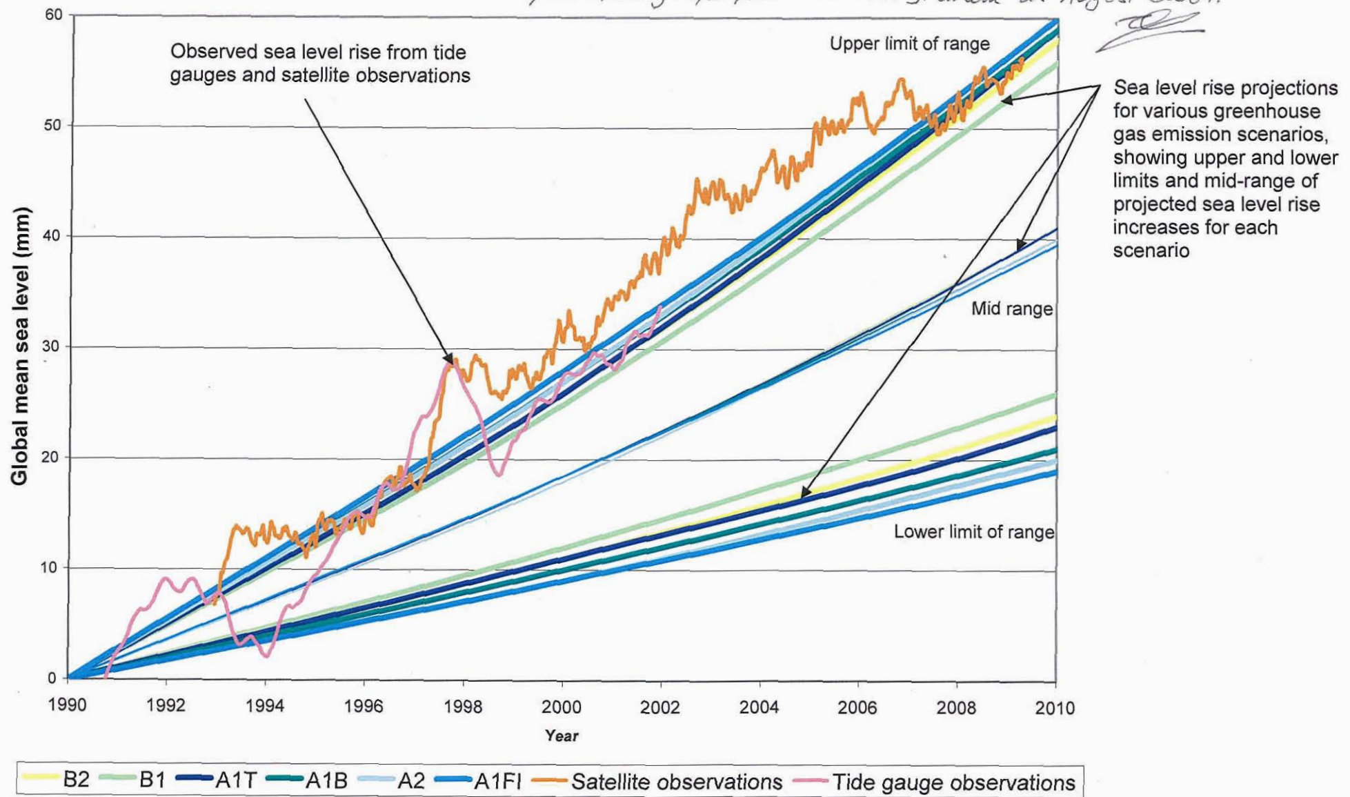
Figure 2 – Projected and observed sea level rise
