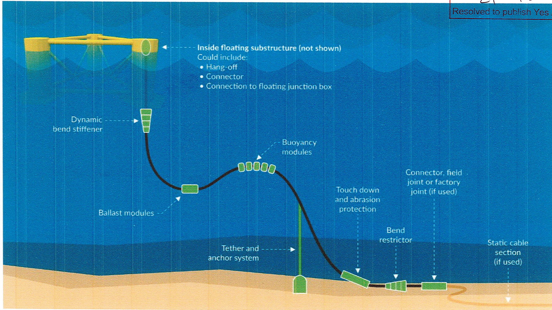
Figure 16 Floating offshore wind dynamic cable system. An actual system would not use all of these elements at the same time. The horizontal distance between the floating substructure and the touchdown point is typically around 200 m. Image courtesy of BVG Associates. All rights reserved.
