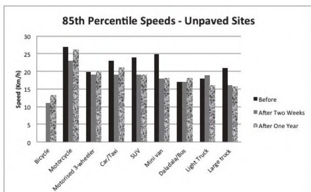
Figure 11. 85 th Percentile Speeds by Vehicle Category (Unpaved Sites)
