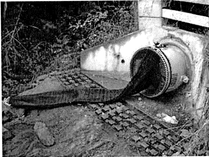
Detachable end-of-pipe trap.
