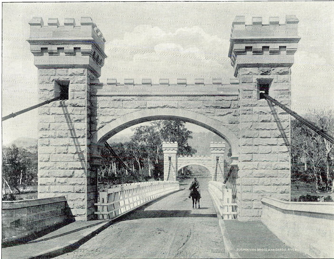
HAMPDEN BRIDGE, OVER KANGAROO RIVER, ON MOSS VALE-NOWRA ROAD. View showing Roadway. Height from Deck to under-side of Arch, 18 ft.
