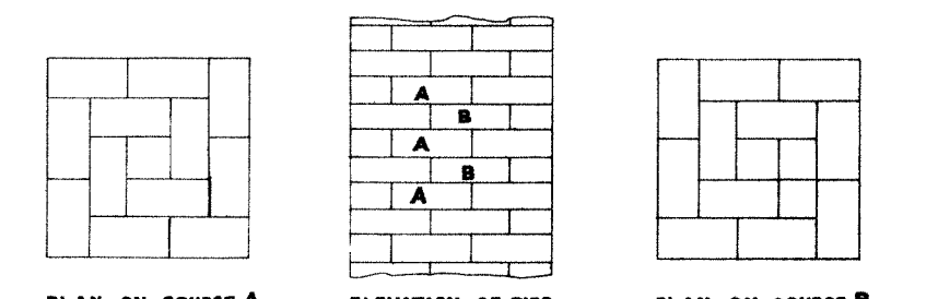
— DETAIL OF PIERS —
