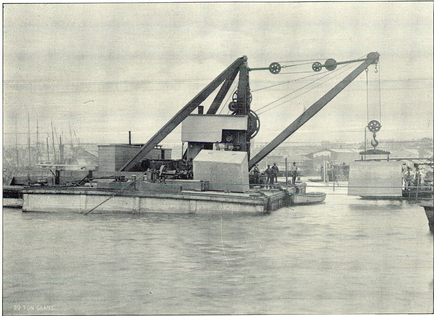
DARLING ISLAND IMPROVEMENTS—30-TON FLOATING BLOCK-SETTING CRANE.
