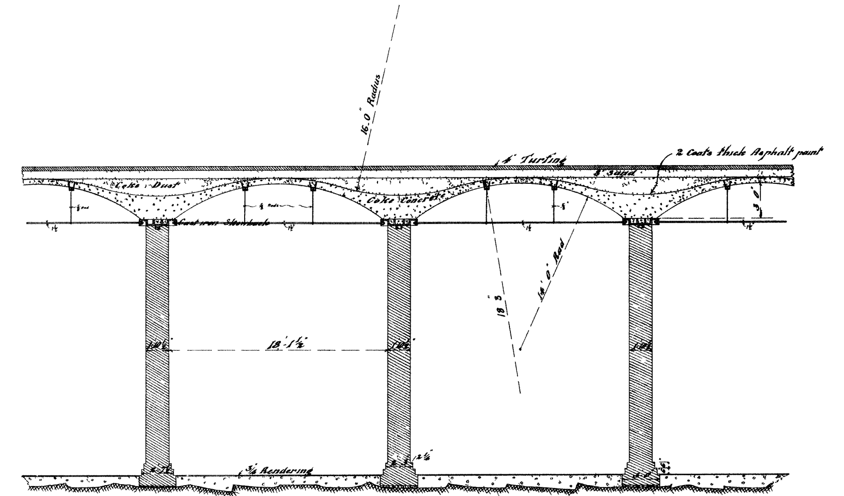
— SECTION ON LINE A.A. —
