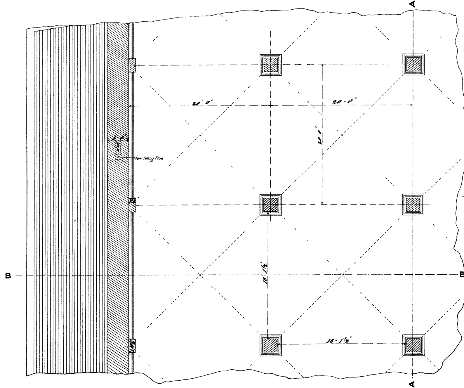
— SECTIONAL PLAN — — OF GROINED ARCHED ROOFING —
