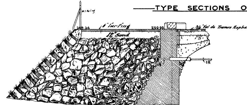
— TYPE SECTION OF TURFING &c —
