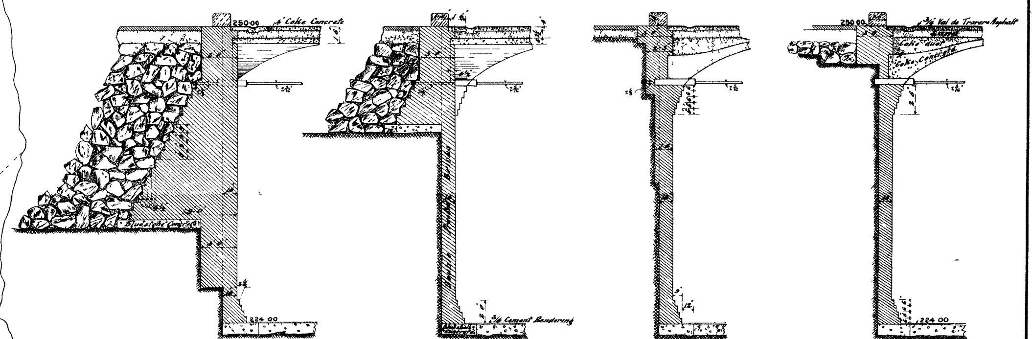
— TYPE SECTIONS OF WALL —
