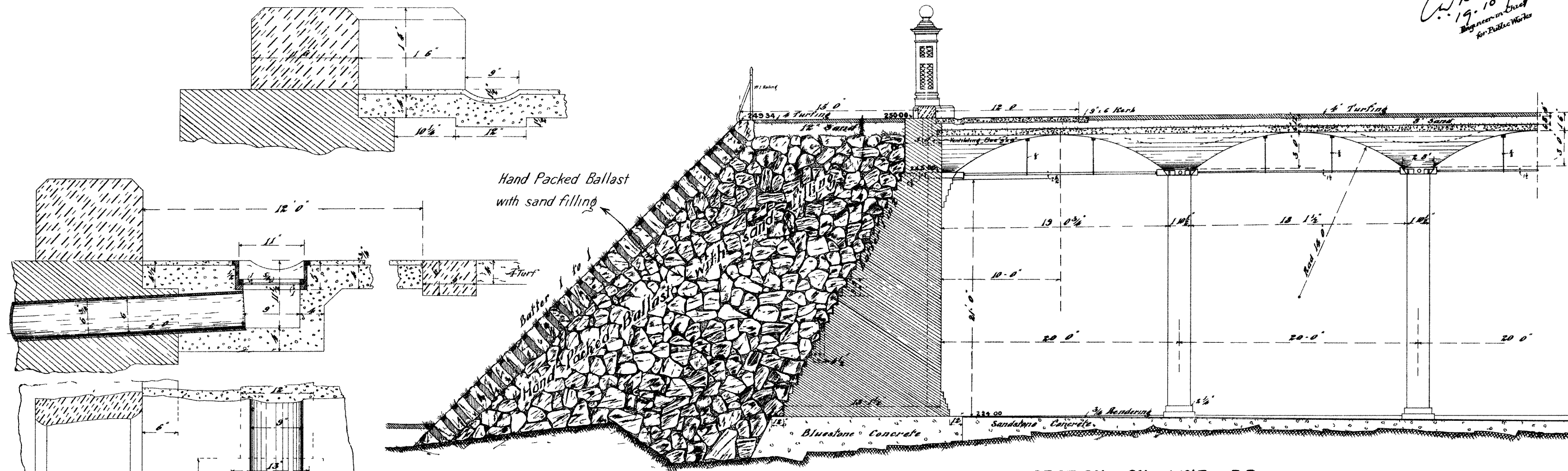
— SECTION ON LINE B.B. —
