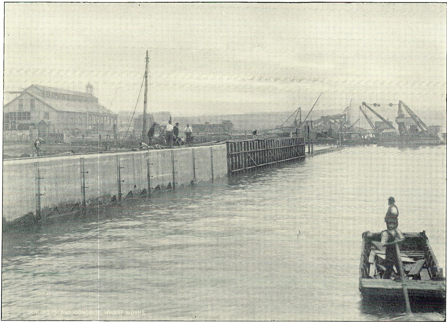
DARLING ISLAND IMPROVEMENTS—CONCRETE WHARF IN COURSE OF CONSTRUCTION, 30-ton Block-setting Crane to right. Depth of water in front of wharf, 28 ft. at low tide.
