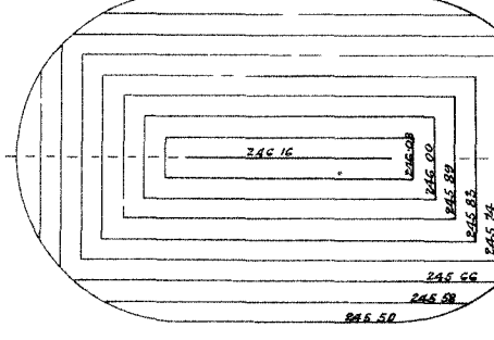
Diagram of Levels of top of Skewbacks
