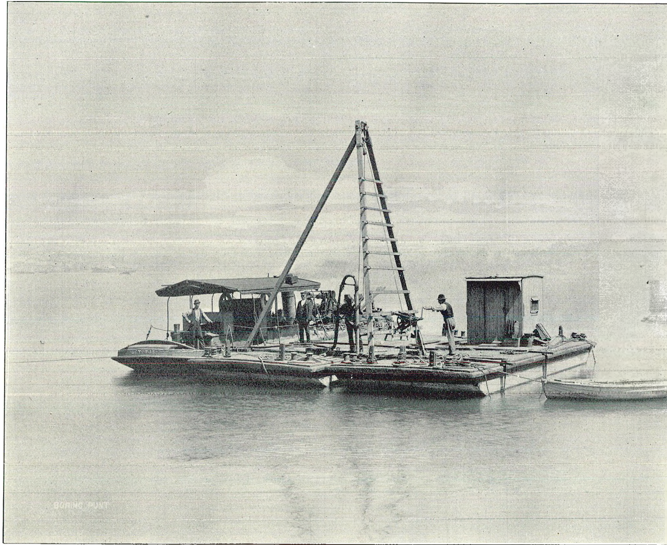
BORING THROUGH BED OF HARBOUR TO ROCK WITH WATER JET.
